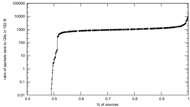
Fig. 1. CDF of the ratio of packets sent to /24s in the 192 /8 to /24s on other /8s.
