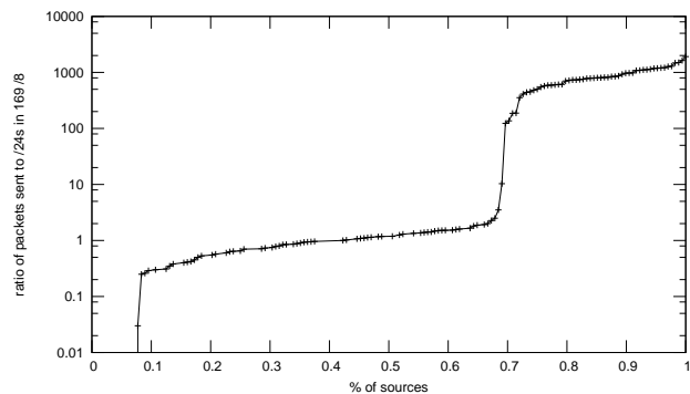
Fig. 2. CDF of the ratio of packets sent to /24s in the 169 /8 to /24s on other /8s.
