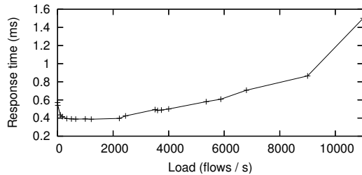
Fig. 6. Flow-setup times as a function of Controller load. Packet sizes were 64B, 128B and 256B, evenly distributed.
