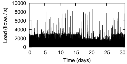
Fig. 7. Flow-request rate for Stanford network.
