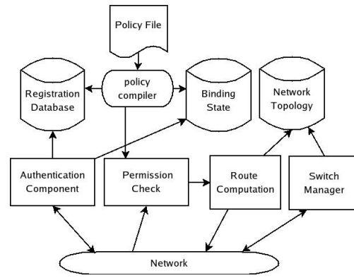
Fig. 3. High-level view of Controller components.
