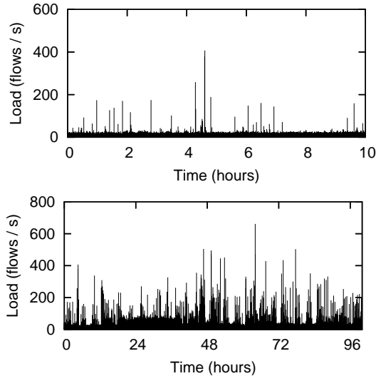
Fig. 5. Frequency of flow-setup requests per second to Controller over a 10-hour period (top) and 4-day period (bottom).
