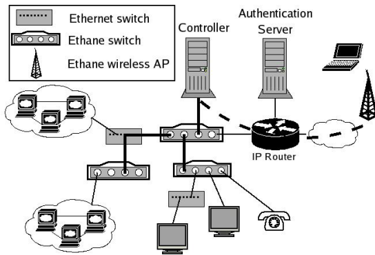
Fig. 2. An example Ethane deployment.
