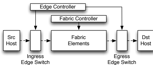
Figure 1: The source host sends a packet to an edge switch, which after providing network services, sends it across the fabric for the egress switch to deliver it to the destination host. Neither host sees any internals of the fabric. The control planes of the edge and fabric are similarly decoupled.
