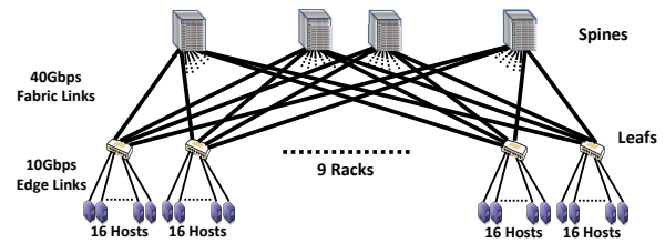
Figure 3: Baseline topology used in simulations.
